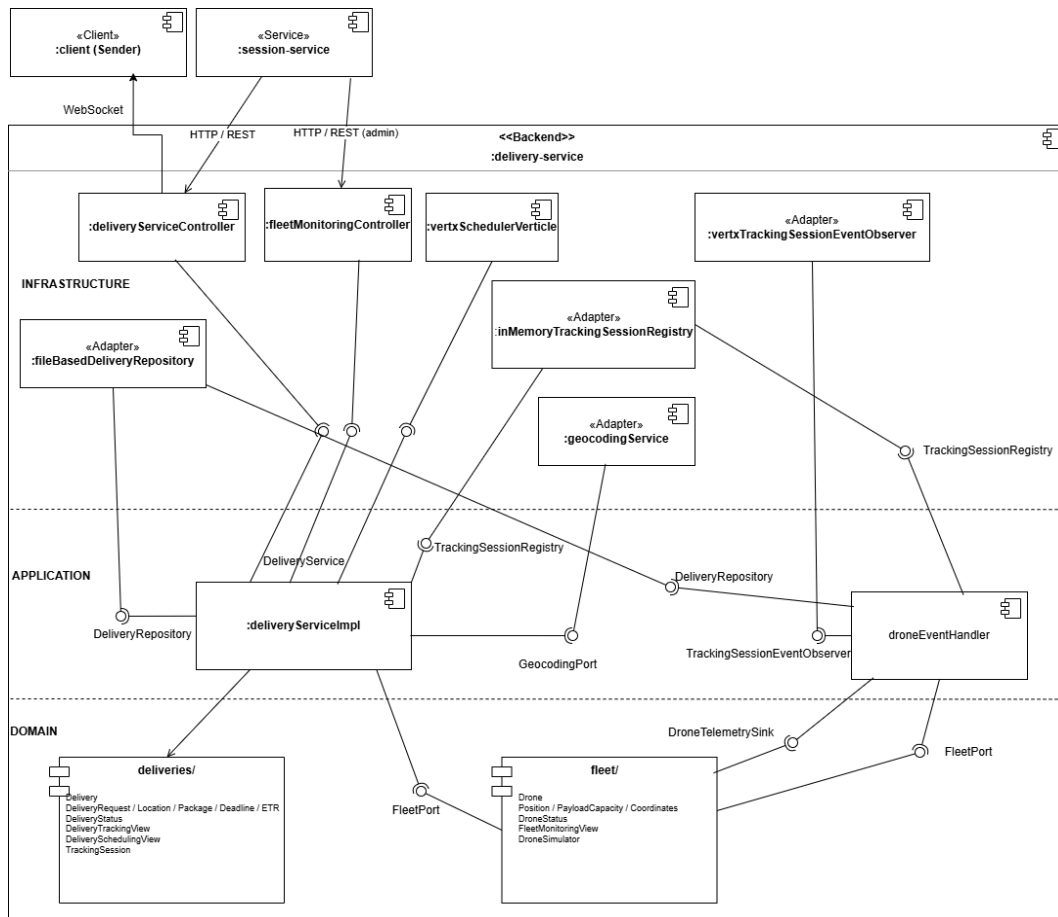
C&C diagram del delivery service (Deliveries + Fleet)
